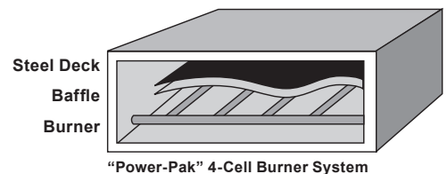
"Power-Pak" 4-Cell Burner System
