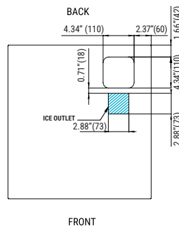
CENTRAL CROSS SECTION VIEW OF THE BASE
