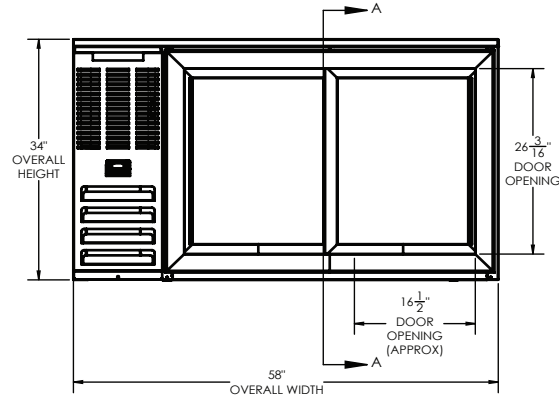
ELEVATION VIEW
