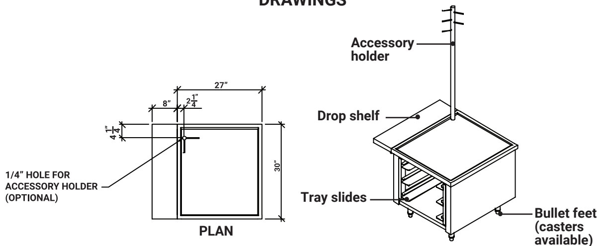
SMS - Universal Slicer/Mixer Stand (shown with options)
