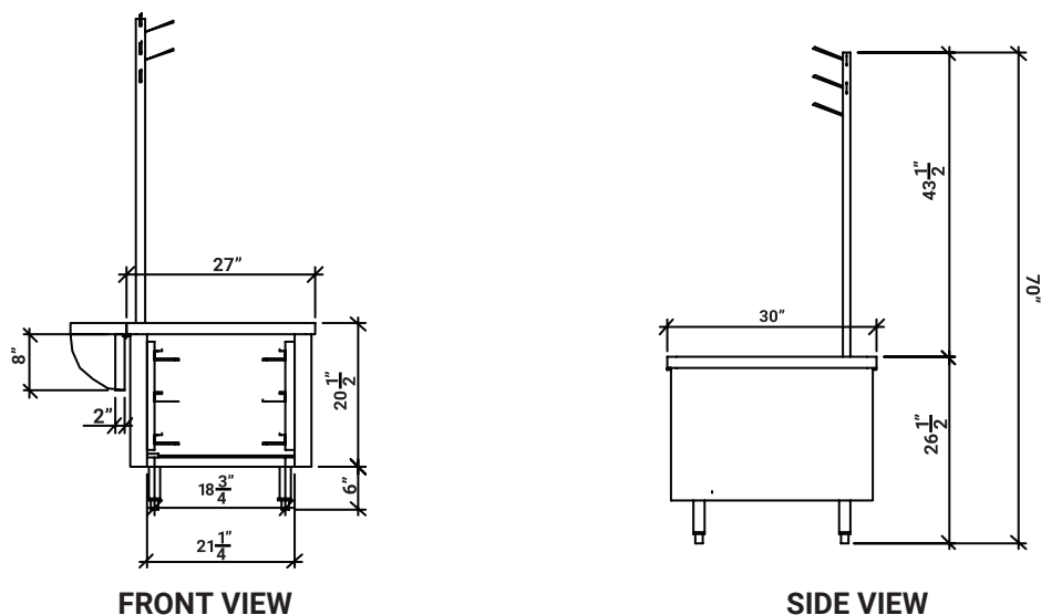
SMS - Universal Slicer/Mixer Stand (shown with options)
