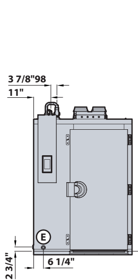
DRAIN POSITION
