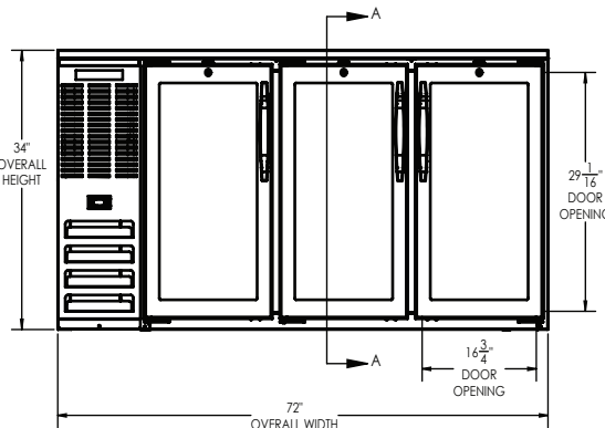
ELEVATION VIEW
