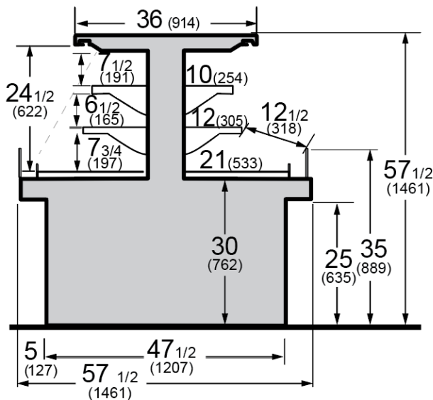
Cross section
