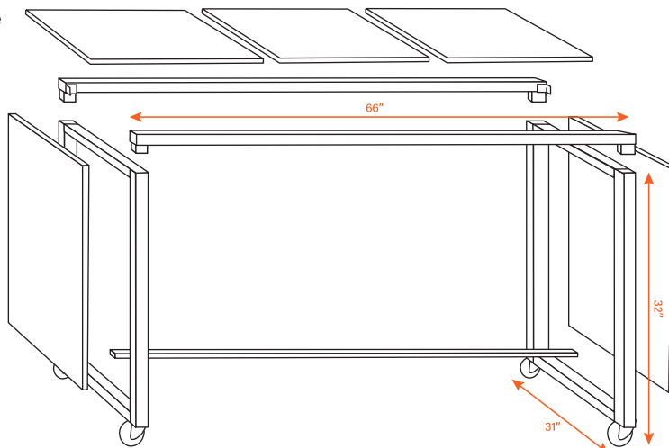
3 Tile Frame Z2020
