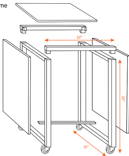
3 Tile Frame Z2020
