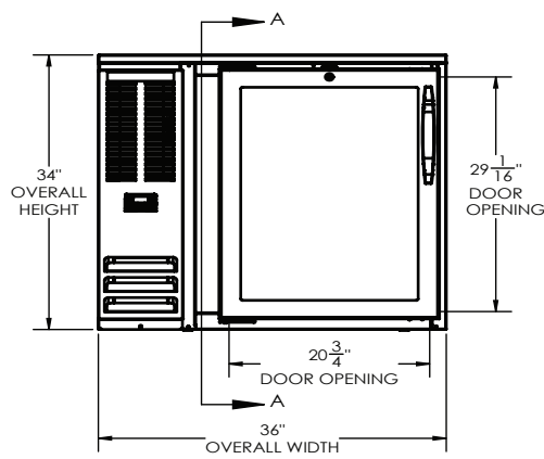
ELEVATION VIEW
