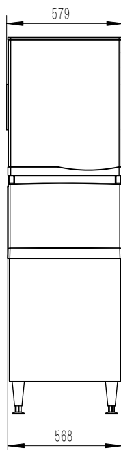
Front View
