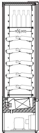
OPTIONAL: S/S ROUND TUBULAR RACK
