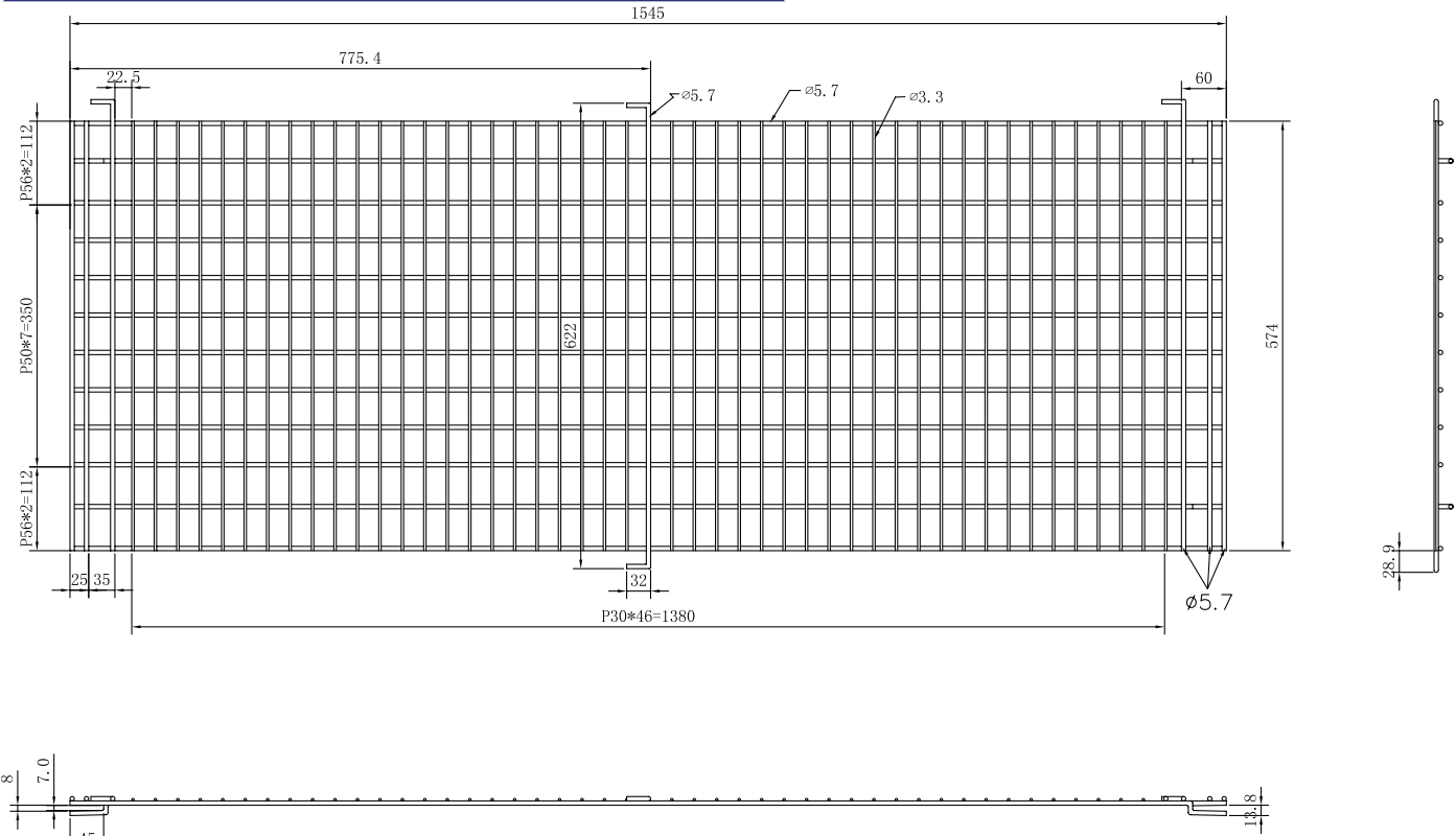
TECHNICAL DRAWING (Side Panel Left)
