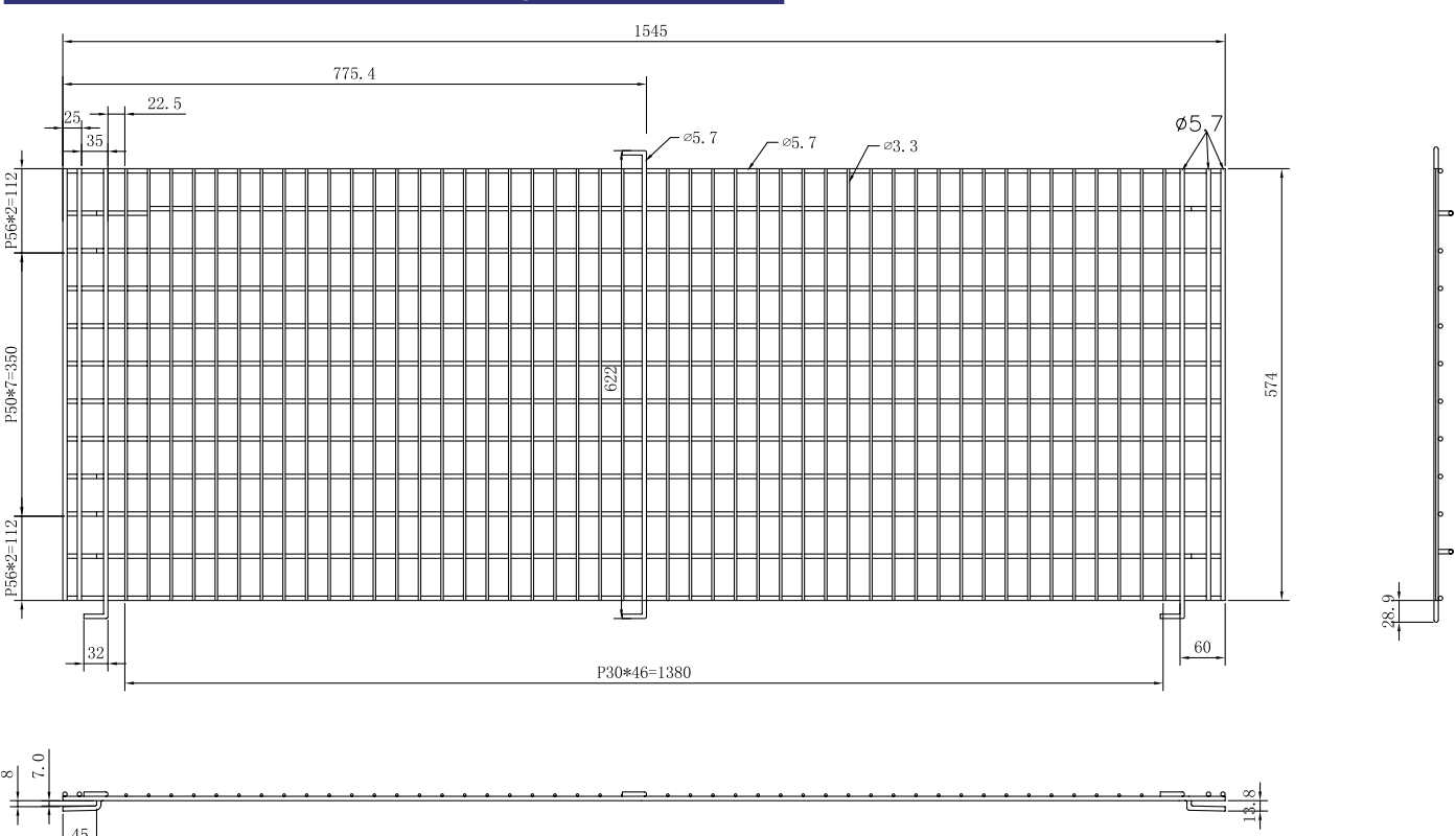
TECHNICAL DRAWING (Side Panel Right)
