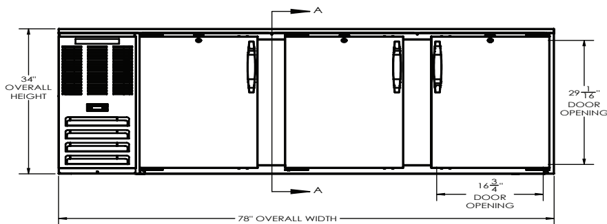
ELEVATION VIEW
