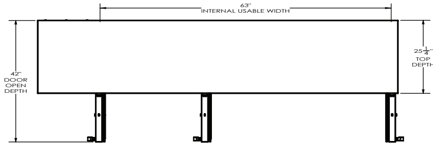
ELEVATION VIEW
