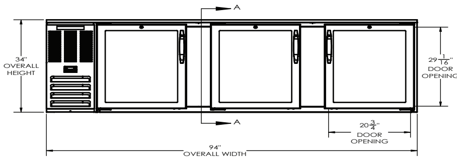
ELEVATION VIEW
