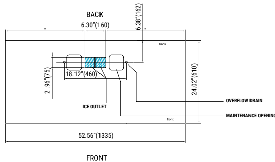
CENTRAL CROSS SECTION VIEW OF THE BASE
