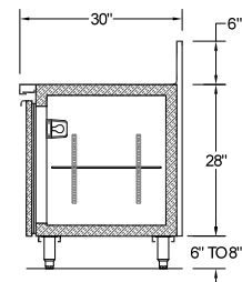
SECTION VIEW
