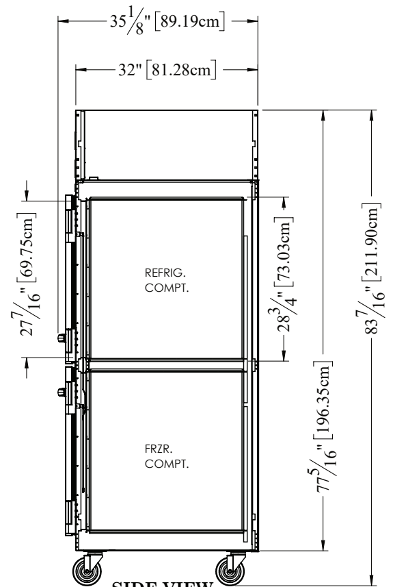
SIDE VIEW
