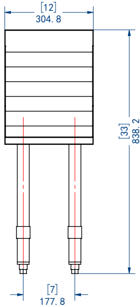
Front View
