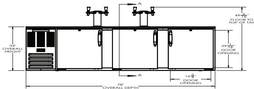
ELEVATION VIEW
