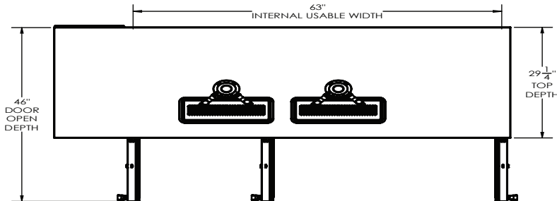
ELEVATION VIEW
