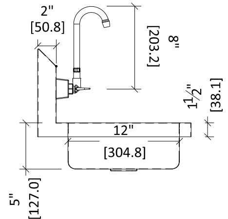
Side Views
