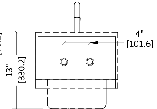
Back Views
