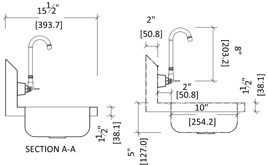
Side Views
