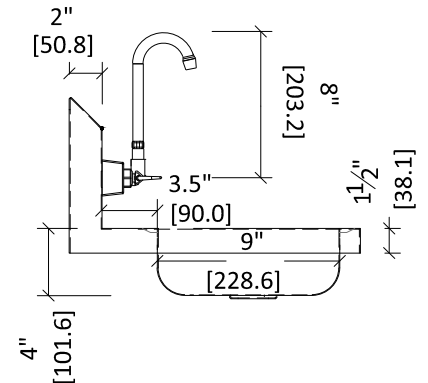
Side Views
