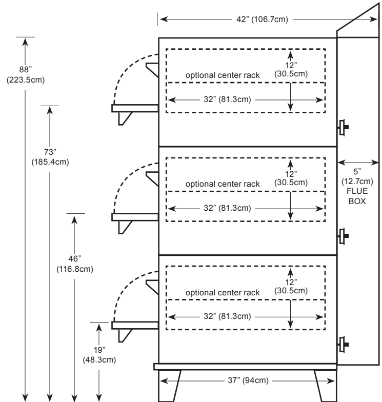
SIDE VIEW CW53BSC
