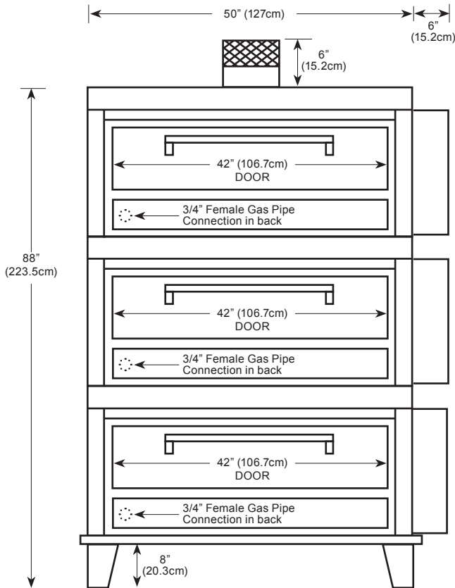
FRONT VIEW CW53BSC
