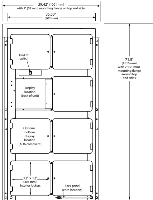
F2GBOB-7 (Standard Ambient Operation) INTERIOR/INSIDE VIEW OPERATOR SIDE
