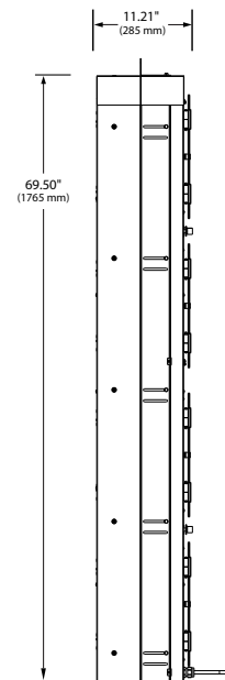
F2GBOB-7 INTERIOR/INSIDE SIDE VIEW OPERATOR SIDE
