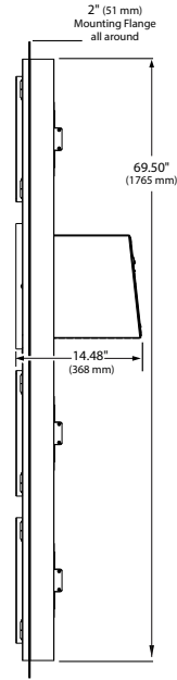
F2GBOF-7 EXTERIOR/OUTSIDE SIDE VIEW CUSTOMER SIDE
