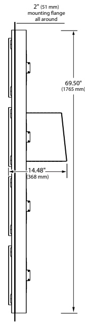
F2GBOF-11 EXTERIOR/OUTSIDE SIDE VIEW CUSTOMER SIDE
