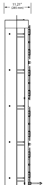
F2GBOB-11 INTERIOR/INSIDE SIDE VIEW OPERATOR SIDE
