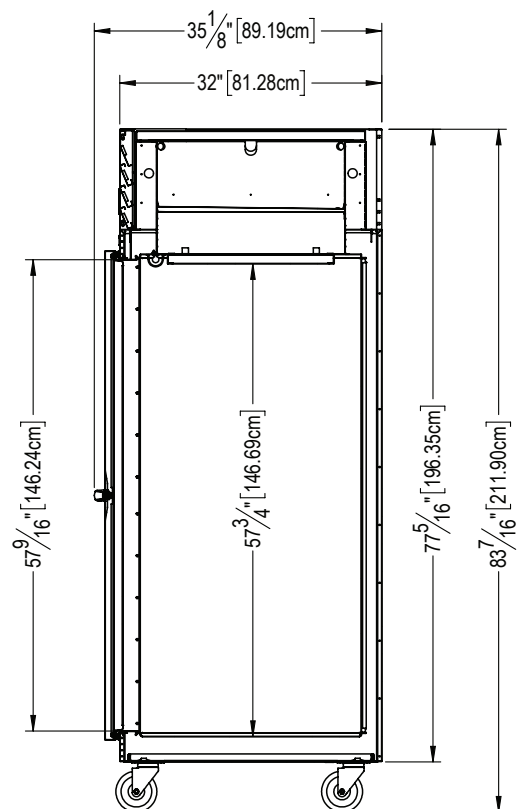
SIDE VIEW
