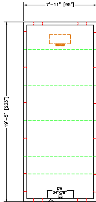
PLAW VIEW LEFT HINGE SELECT
